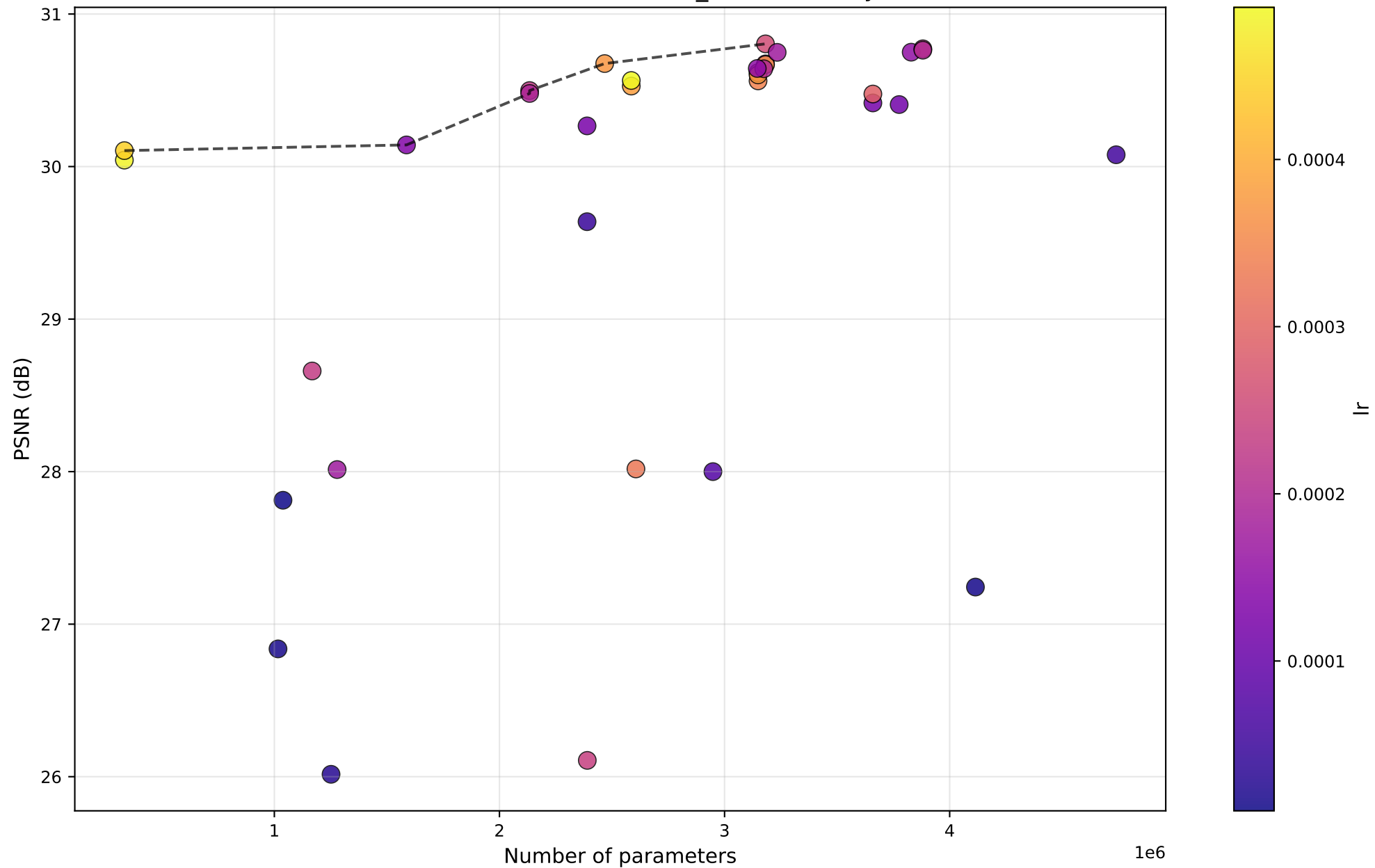
PSNR vs #Params — DHTCUN_baseline — by lr
